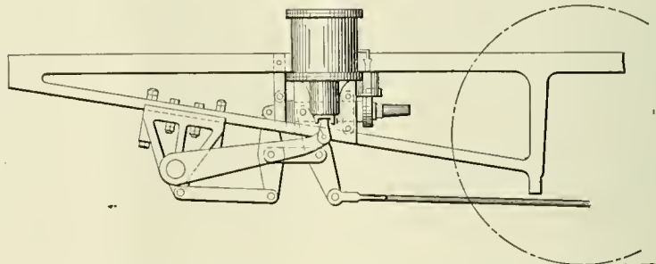
ARRANGEMENT OF SLACK ADJUSTER FOR DRIVER BRAKES.
